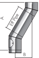
30° offset using Inspection Bend
