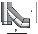
Offsets for 135° Tee & 45° Bend
