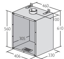
Recessed Flue Box
