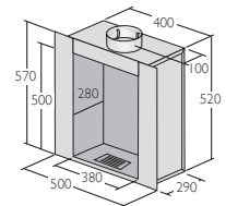
VRV Twin Wall Flue Box
