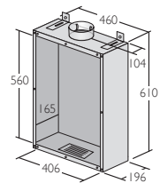
Standard Flue Box
