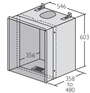
Large Flue Box for back boiler
